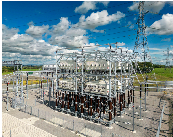
Figure 7. SSSC at National Grid, UK (Smartwires)
